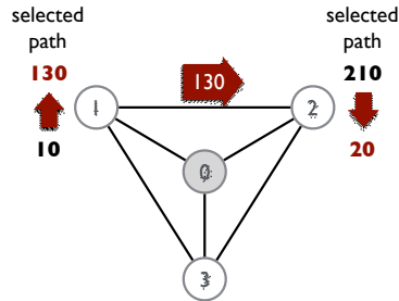
Fig. 2: Route selection with “disagreeing” AS policies is non-monotonic.
