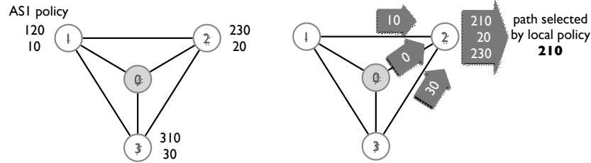
Fig. 1: (left) Example: the SPP model for AS policies. (right) Policy-based route selection.
