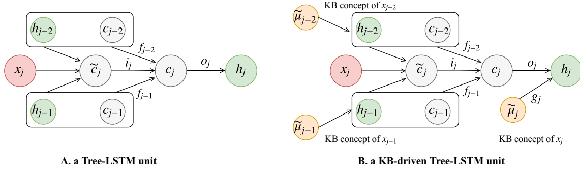
Figure 2: (A): a Tree-LSTM unit. (B): a KB-driven Tree-LSTM unit. The yellow circles denote external KB concept embeddings.
