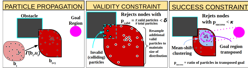
Fig. 2 The uncertainty of the system is captured using a particle distribution over the system's state. Using the black-box propagation model, each particle is propagated to obtain the next state's distribution (left). In order for the new node to be added to the tree, two robustness constraints are checked. First, the ratio of valid particles over the total must exceed the threshold \delta (middle). Validity can refer to constraints such as being collision-free, or other criteria, depending on the system. Second, the most dense cluster of particles is computed through mean-shift, and the goal region is transposed to this center (right). The ratio of particles that lie within this transposed region must exceed the threshold \kappa .
