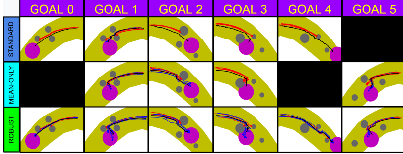
Fig. 5 Physics engine simulation results for manipulating the underactuated hand between obstacles (in gray). The black curves are the planned paths to the goal region (magenta circle). The blue and red curves are successful and failed paths, respectively. The yellow region is the approximated workspace of the hand. Black cells indicate that a solution was not found.
