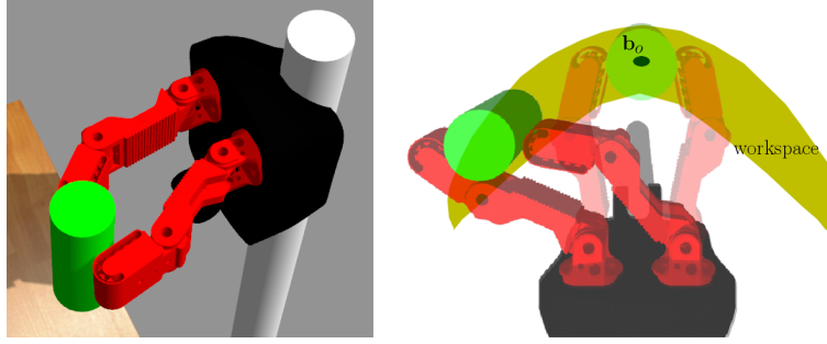
Fig. 1 Physics engine simulation of the Model T42 adaptive hand in the Gazebo environment (left). A visualization of the approximated workspace (based on data) of the hand, shown in yellow, along with the initial belief distribution \mathbf{b}_0 (right).
