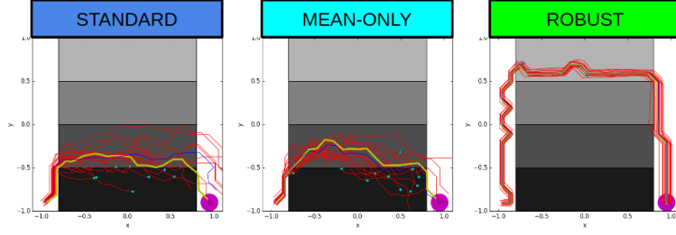
Fig. 4 Experimental results for the point-system showing plots of the planned path vs. multiple rollouts for the STANDARD (left), MEAN-ONLY (middle), and ROBUST (right) algorithms.
