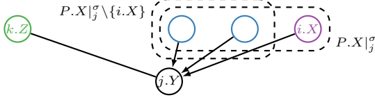
Figure 3: Non-RBO with P.X \rightarrow \mathcal{V}_Y and Q.Z \perp \mathcal{V}_Y
