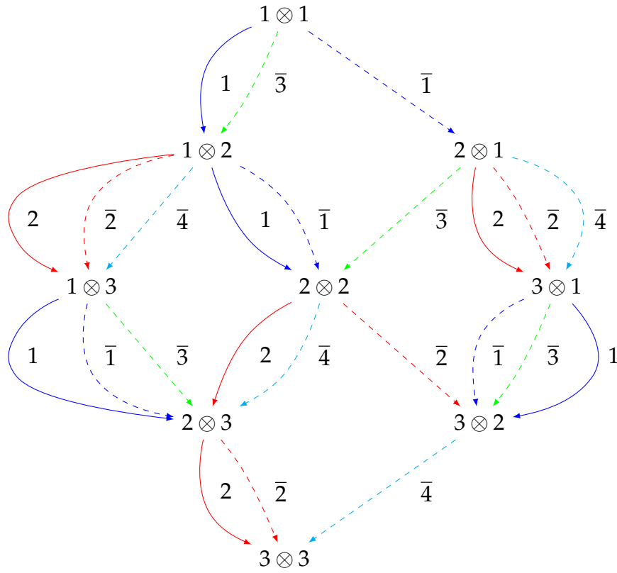
Figure 2: The crystal \mathcal{B}^{\otimes 2} of type \mathfrak{q}(3) of Example 3.2 .
