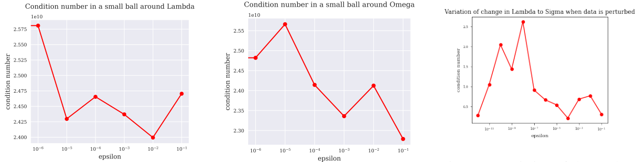
Figure 7: Variation of the randomized condition number as a function of the perturbation error on the sociology dataset
