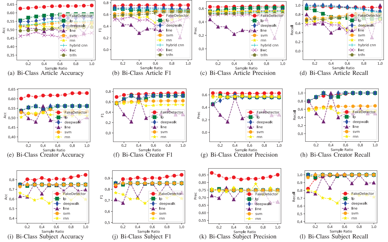
Fig. 5. Bi-Class Credibility Inference of News Articles 5(a)-5(d), Creators 5(e)-5(h) and Subjects 5(i)-5(l).
