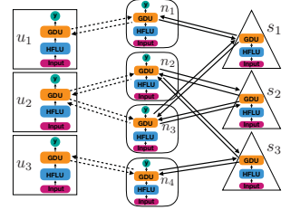
Fig. 4. The Architecture of Framework FAKEDETECTOR.
