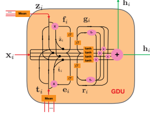
Fig. 3. Gated Diffusive Unit (GDU).
