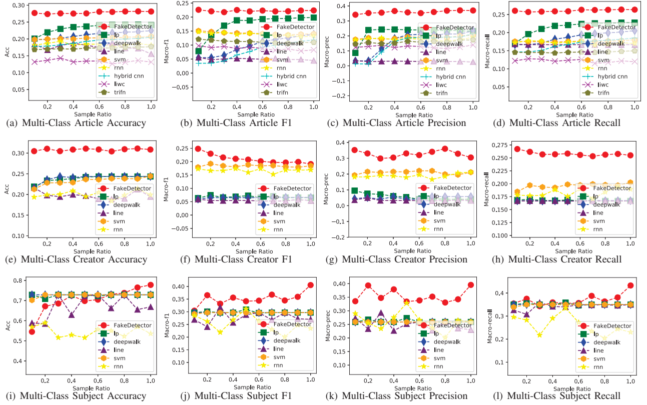
Fig. 6. Multi-Class Credibility Inference of News Articles 6(a)-6(d), Creators 6(e)-6(h) and Subjects 6(i)-6(l).
