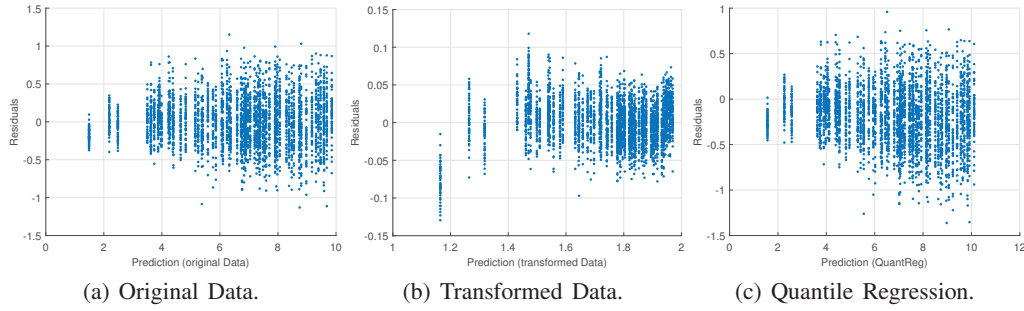
Figure 3: Residuals against predictions for the quadratic model case.
