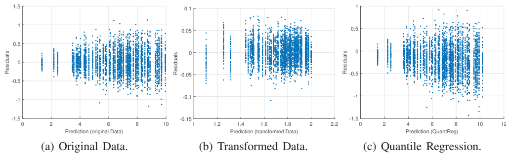
Figure 4: Residuals against predictions for the cubic model case.
