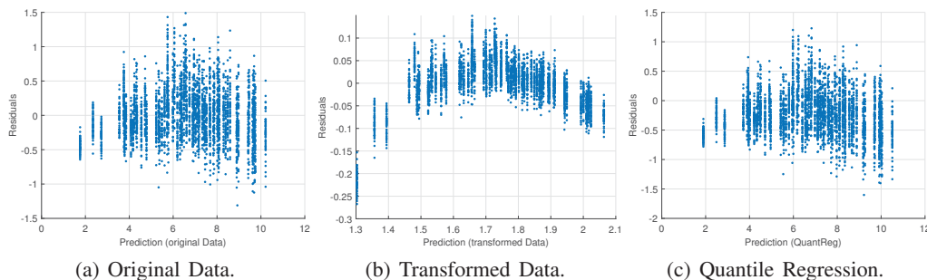
Figure 2: Residuals against predictions for the linear model case.
