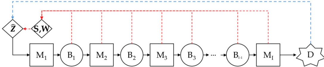
Figure 1: Job flow and information flow for a control point policy.
