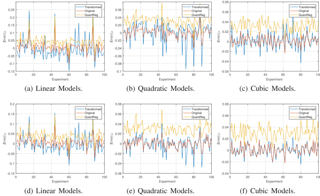
Figure 5: Relative error for part type 1 (Figure 5a-5c) and part type 2 (Figure 5d-5f).
