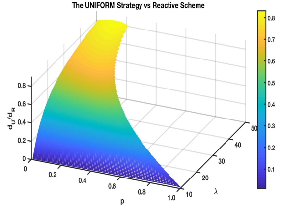
Fig. 11. Theoretical Delay Comparison between UNIFORM Strategy and Reactive Scheme
