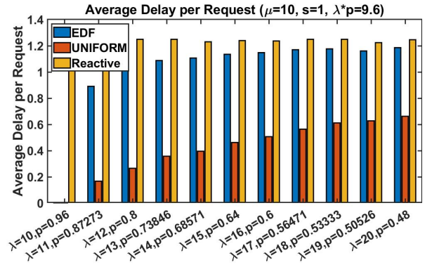
Fig. 8. Comparisons among EDF, UNIFORM and Reactive Schemes: \lambda p = 9.6
