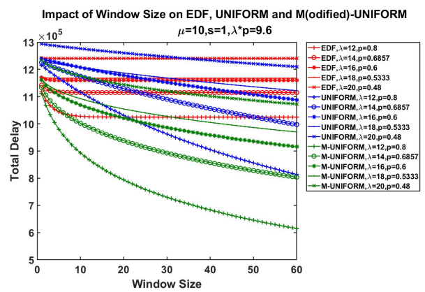
Fig. 13. Comparisons among EDF, UNIFORM and Modified-UNIFORM: \lambda p = 9.6
