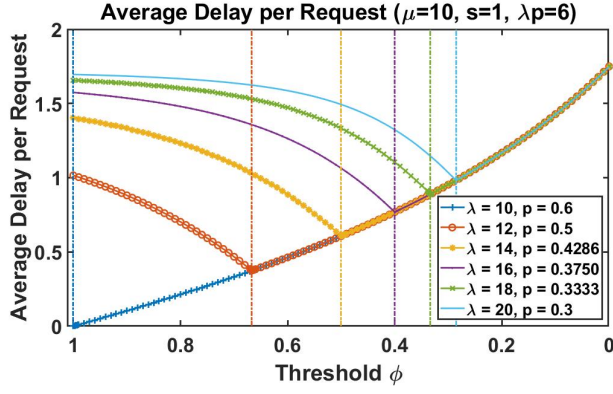
Fig. 5. Comparisons among threshold-based methods: \lambda p = 6
