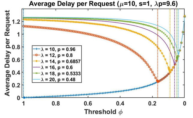
Fig. 6. Comparisons among threshold-based methods: \lambda p = 9.6
