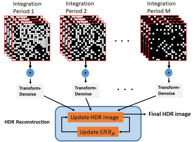
Figure 1. HDR Reconstruction pipeline. The raw QIS frames are summed and denoised. Then the denoised images are combined according to the weights proportional to SNR_H . (See Section 3 for details.)
