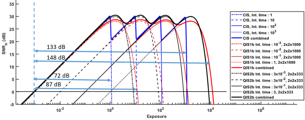
Figure 2. Comparison of Exposure referred signal-to-noise ( \text{SNR}_H ) for CIS and QIS. (QIS1b: Single-bit QIS, QIS2b: Two-bit QIS). Ideal QIS and CIS are considered, i.e. the read noise is assumed to be zero in both cases. CIS is assumed to have a full well capacity of 4000 electrons. For single-bit QIS, binning of 1000 frames with 2 \times 2 spatial oversampling is assumed. For 2-bit QIS, T = 333 frames with 2 \times 2 spatial oversampling is assumed. QIS has a larger dynamic range than CIS for each exposure, and has a more consistent SNR over the entire range when the low dynamic range images are combined to get a single high-dynamic range image.
