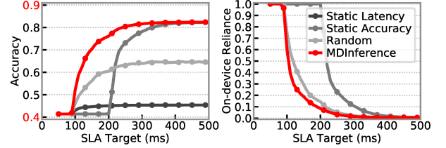
Fig. 7: Aggregate accuracy and on-device model reliance on residential network. MDINFERENCE demonstrated improvements throughout all tested SLAs. At lower SLAs MDINFERENCE can quickly improve the aggregate accuracy. Meanwhile, MDINFERENCE also reduces the reliance on on-device models at low SLAs, much more quickly than other algorithms.
