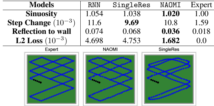
Figure 10: Billiard Forward Prediction Comparison. Top: metrics for billiards prediction accuracy. Statistics closer to the expert indicate better model performance. Bottom: predicted billiards trajectories. Black dots represent known observations. NAOMI perfectly recovers the ground-truth.
