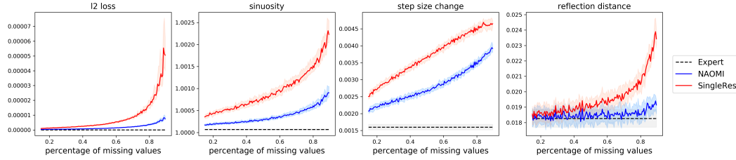
Figure 6: Billiards model performance with increasing percentage of missing values. The median and 25, 75 percentile values are displayed at each number of missing steps. Statistics closer to the expert indicate better performance. NAOMI performs better than SingleRes for all metrics.
