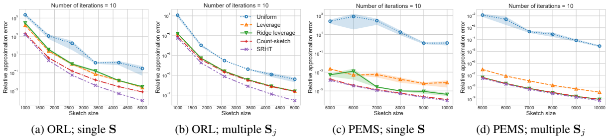
Figure 4: Relative approximation error vs. sketch size on ORL and PEMS after 10 iterations. Single S : using a single sketching matrix \mathbf{S} throughout the iterations. Multiple \mathbf{S}_j : sample a new \mathbf{S}_j at every iteration j . Errors are on log-scale; note the difference in magnitude of the approximation errors across plots.
