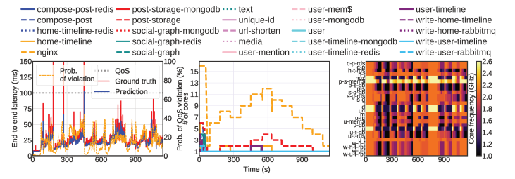
Fig. 3: Latency and resources under a diurnal load.
