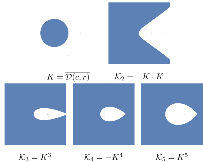
Figure 4: Our region K = \overline{\mathcal{D}(c, r)} , \mathcal{K}_2 , \mathcal{K}_3 , \mathcal{K}_4 and \mathcal{K}_5 in the case of \beta = 4 and \gamma = \frac{1}{2} . Here, the intercept of \mathcal{K}_d on the positive real line is minimised at d = 4 for all d \geq 2 .
