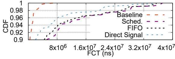
Figure 19: CDF of FCT for datacenter flows > 10KB using HPCC for WAN and datacenter traffic.
