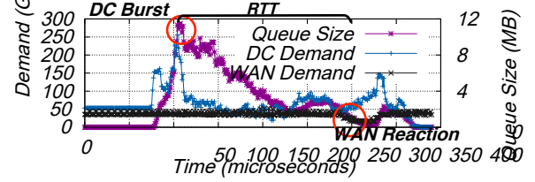
Figure 2: WAN flows start reacting to a burst in demand much later than the burst had occurred and datacenter flows have already reduced their rate.
