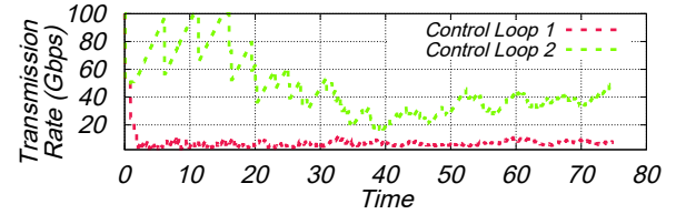
Figure 23: Rate deduced by each control loop when bottleneck 1 has 100 flows going through it while control loop 2 has 10 flows going through it.
