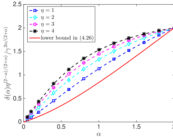
FIGURE 4.3. Comparison of the lower bound in (4.26) (solid line) and numerical results (dashed lines) for the fundamental gap \delta(\alpha) of the FSO (1.5) with V(x, y) = \gamma^2(x^2 + \eta^2 y^2) for different \eta \geq 1 and \gamma > 0 .
