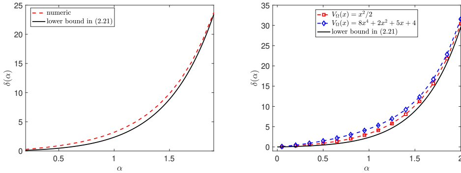
FIGURE 3.2. Comparison of the lower bound in (2.21) (solid line) and numerical results (dashed lines) for the fundamental gap \delta(\alpha) of the FSO (3.1) with n = 1 , \Omega = (0, 1) and V_\Omega(x) \equiv 0 (left) or different convex potentials V_\Omega(x) (right).
