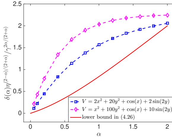
FIGURE 4.4. Comparison of the lower bound in (4.26) (solid line) and numerical results (dashed lines) for the fundamental gap \delta(\alpha) of the FSO (1.5) with different potentials V(\mathbf{x}) .
