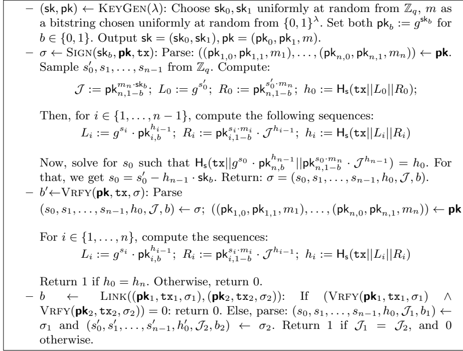
Fig. 2: Construction of DLSAG. For ease of exposition, we assume that the secret key sk_b corresponds with the public key pk_{n,b} . As noted before, the position of the true signer's public key is chosen uniformly random.
