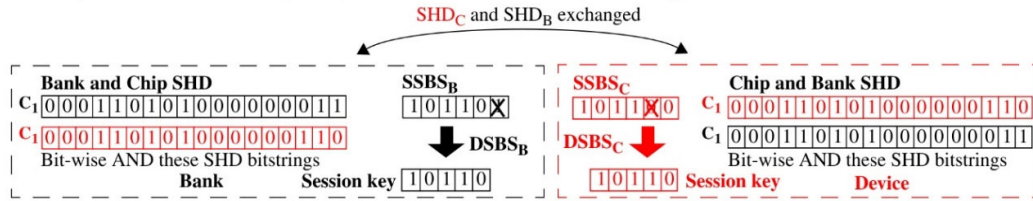
DHD_Key: Construct and exchange SHD, construct SSBS and DSBS (Session keys)
