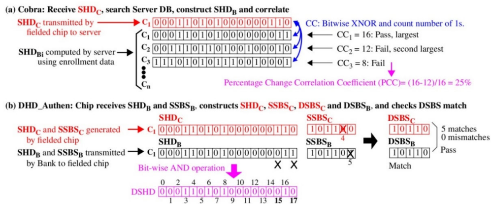
Figure 4. Bit-string construction algorithms (a) Cobra for device authentication and (b) DHD_Authen for server authentication.
