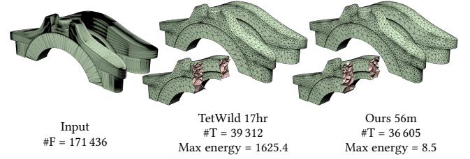
Fig. 17. Example of a challenging model where fTETWILD is 17 times faster than TetWild.
