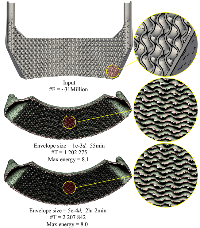
Fig. 23. Meshing a complex model with 93 million vertices and 31 million faces with different envelope sizes (top). The input mesh contains degenerate triangles and severe self-intersections. Our output tetrahedral meshes are in geometric high quality with either default envelope size (middle) or half envelope size (bottom).
