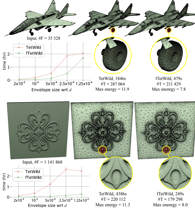
Fig. 15. Input models and running time plots of fTETWILD and Tetwild with \epsilon reduced from 2 \cdot 10^{-3}d to 1.25 \cdot 10^{-4}d (left). Output tetrahedral meshes of the two methods at \epsilon = 5 \cdot 10^{-4}d (middle and right). Note that we flipped all the normals of the input triangles of the airplane model for visualization purposes (see Figure 30 for a detailed discussion).
