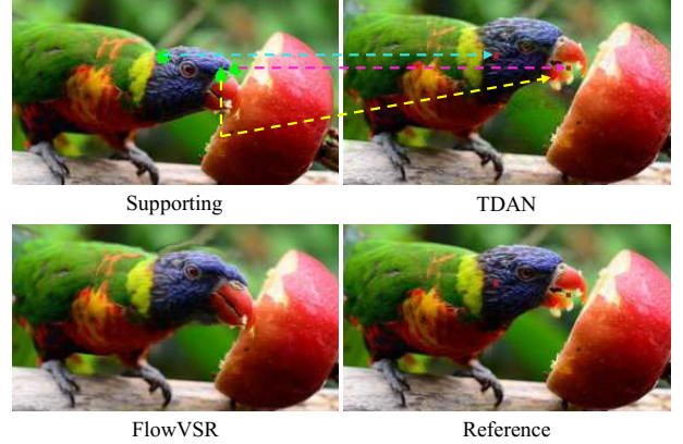
Figure 6. Temporal alignment results of FlowVSR and TDAN on a supporting/reference frame pair with a very large temporal gap (60 frames). The TDAN can exploit rich image contexts containing similar content (green regions) as target pixels (red points) from the supporting frame to employ accurately temporal alignment. Note that the alignment is performed on feature maps of supporting frames, so the real exploited image regions for alignment will be much larger than the green regions.
