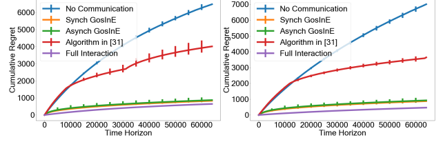
Figure 4: (N, K) are (10, 30) and (15, 40) respectively.
