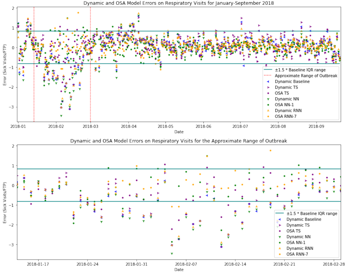
Figure 3: Scatter plot comparing each model’s errors (Baseline blue, TS purple, NN green, RNN orange; Dynamic Y OSA \cdot ) on respiratory visits only. Teal lines highlight outliers compared to the baseline. The underpredictions during the approximate range of the outbreak (in red) are nearly all due to respiratory visits.
