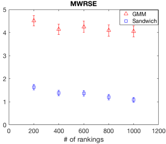
Figure 2: MWRSE with 95% confidence intervals and runtime for 4-RUM over 15 alternatives. We use 5 EM iterations for the sandwich algorithm. Values are averaged over 900 trials. The ground truth for each component ranges between 0 and 10.
