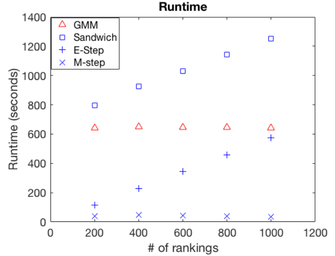
Figure 2: MWRSE with 95% confidence intervals and runtime for 4-RUM over 15 alternatives. We use 5 EM iterations for the sandwich algorithm. Values are averaged over 900 trials. The ground truth for each component ranges between 0 and 10.
