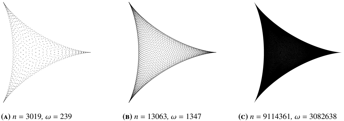
Figure 4: Sometimes G(n, \omega) appears to “fill out” the image of a Laurent polynomial g : \mathbb{T}^{\varphi(d)} \rightarrow \mathbb{C} . Here g(z_1, z_2) = z_1 + z_1 + 1/(z_1 z_2) .
