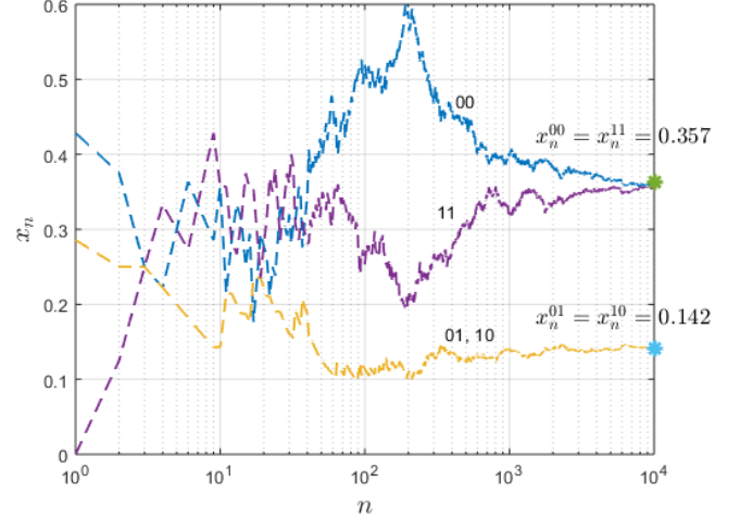
Figure 2. 2-mer frequencies vs the number of mutations in a tandem duplication and substitution system, with \mathcal{A} = \{0, 1\} , s_0 = 0100010 , q_0 = \frac{1}{4} , and q_1 = \frac{3}{4} .
