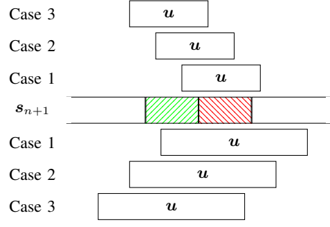
Figure 1. Possible cases for new occurrences of u in s_{n+1} . Cases above and below s_{n+1} correspond to \ell + 1 \leq k < 2\ell and k \geq 2\ell , respectively. The hatched boxes, from left to right, are the template and the copy.
