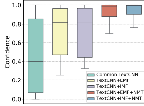
(a) TextCNN on Abuse
