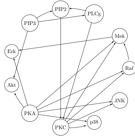
Figure 10: Consensus network, according to Sachs et al. (2005).
