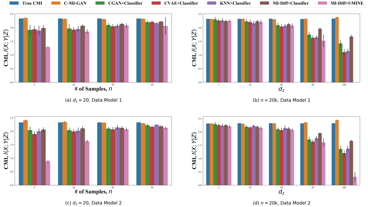
Figure 2: Performance of CMI estimators on the dataset generated using linear models. (a) Model 1: CMI estimates with fixed d_z = 20 and variable sample size, (b) Model 1: CMI estimates with fixed sample size, n = 20k and variable d_z , (c) Model 2: CMI estimates with fixed d_z = 20 and variable sample size, (d) Model 2: CMI estimates with fixed number of samples, n = 20k and variable d_z . Average over 10 runs is plotted. Variation in the estimates are measured using standard deviation and are highlighted in the plots using the thin dark lines on top of the bar plots. The proposed method, C-MI-GAN provides closer estimate of the true CMI, while the state of the art estimators largely underestimate its value. C-MI-GAN outperform the state of the art methods in terms of variation in estimates as well. (Best viewed in color)
