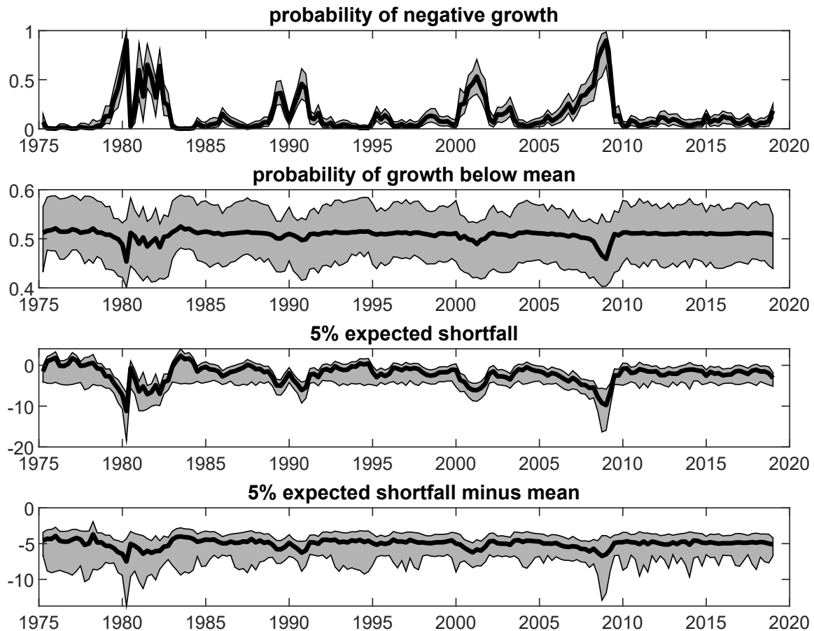
Figure 11: U.S. factor model: Recession probability and expected shortfall, one
