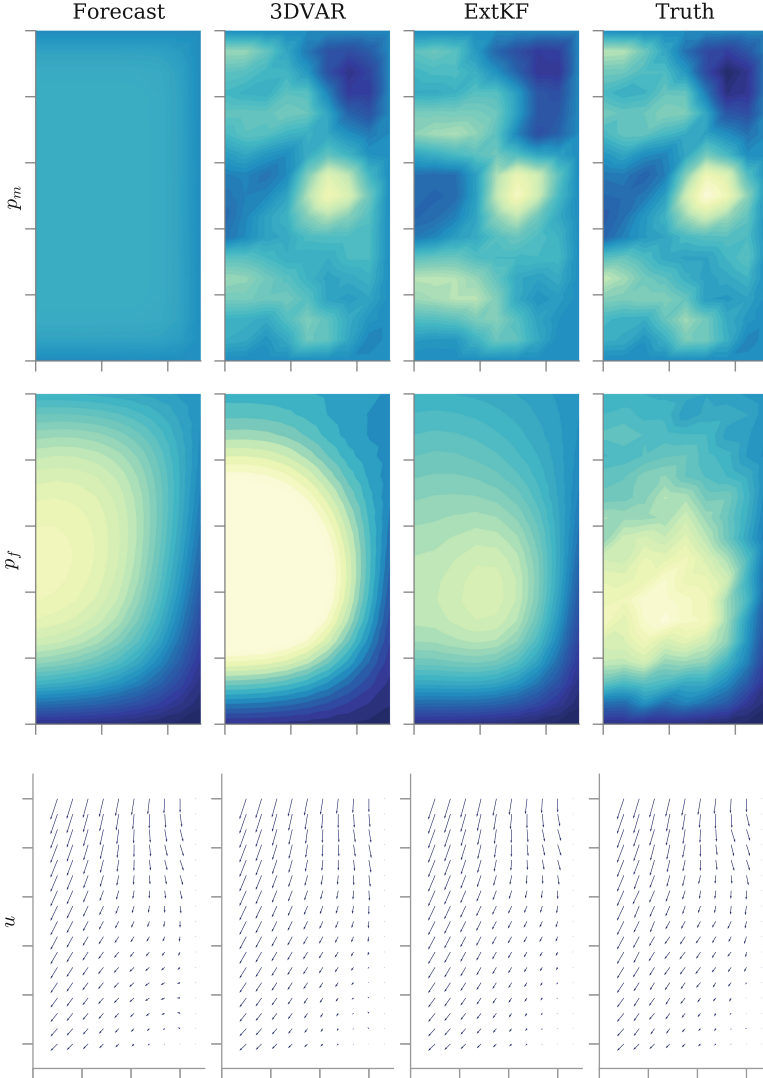
Fig. 6. Results of filters at time t = 0.02 in the 2D model.
