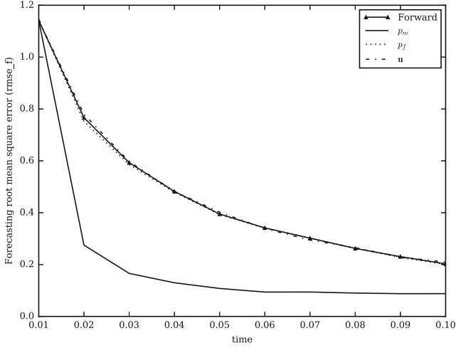
Fig. 7. Forecasting error of Kalman Filter with different observations.
