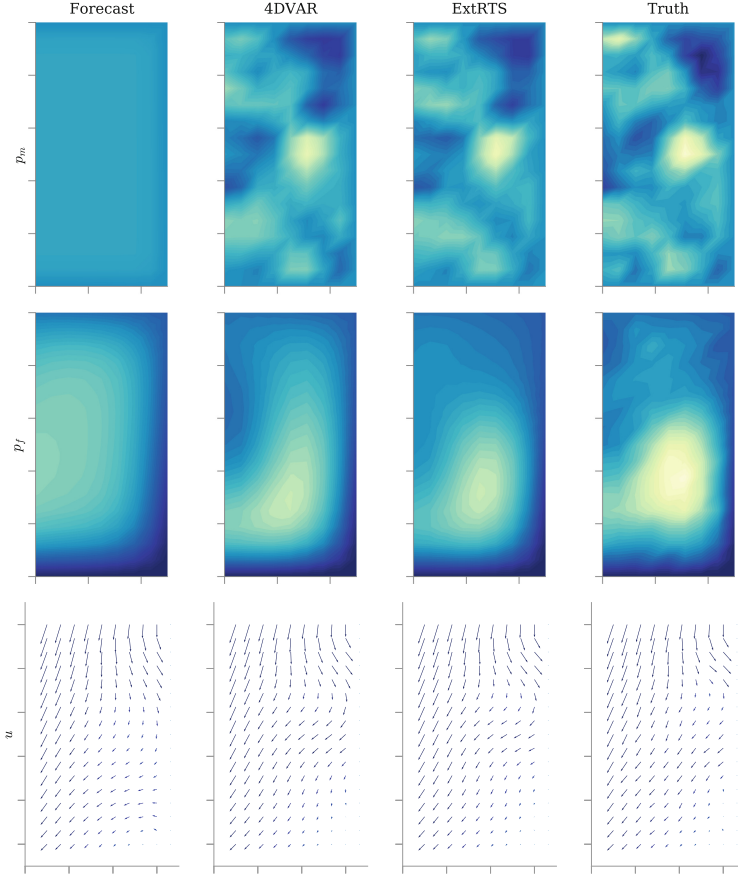
Fig. 5. Results of smoothers at time t = 0.01 in the 2D model.
