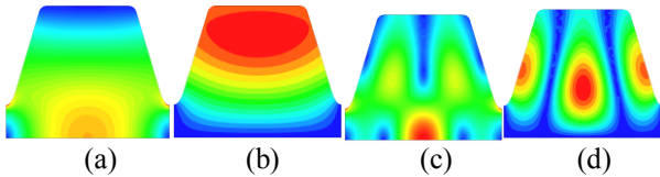
Fig. 1.(a) Bimodal cavity electric and (b) magnetic field distributions for TM010 mode; (c) electric and (d) magnetic field distributions of its 3 rd harmonic TM012 mode.
