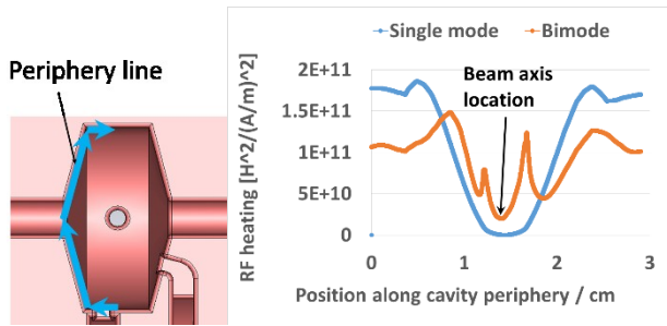
Fig.8. Comparison of RF pulsed heating (proportional to \langle H^2 \rangle ) for our cavity operated with one mode and bimodally, plotted along the cavity periphery. Both cases are for a peak accelerating gradient of 256 MV/m.
