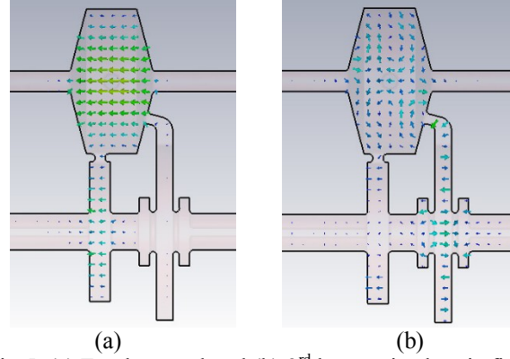
Fig.5. (a) Fundamental and (b) 3 rd harmonic electric field distributions. Both modes have Q of about 7400.
