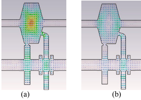
Fig.7. (a) Electric field distributions at the center point at its peak field gradient (256 MV/m); and (b) its zero field gradient.
