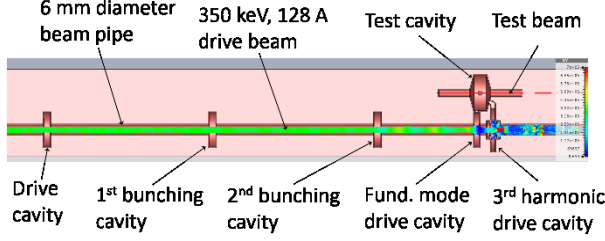
Fig.3. Top view of the half split of the cavity system.
