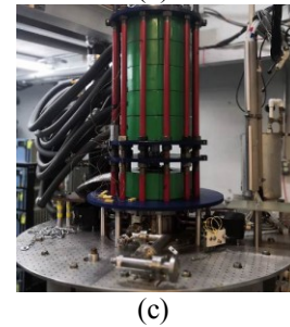
Fig. 2. (a) Engineering design of the test stand setup. (b) End-to-end tracking simulation of beam and magnetic field distribution along axis. (c) Assembled test stand, showing magnetic system on top of 500kV/218A gun tank.
