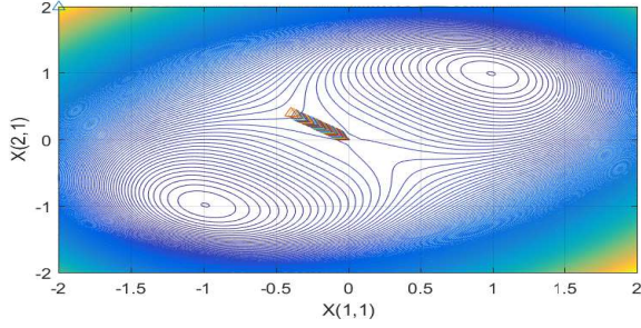
(a) GD in the contour lines of h_\mu(X) with \mu = 0.01
