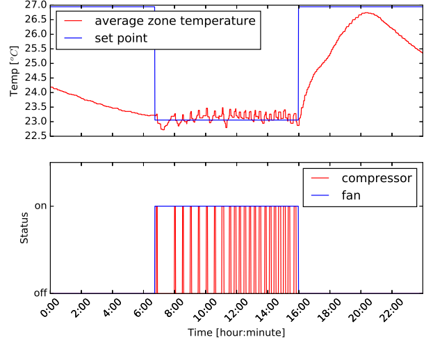
Figure 2: Typical RTU operation
