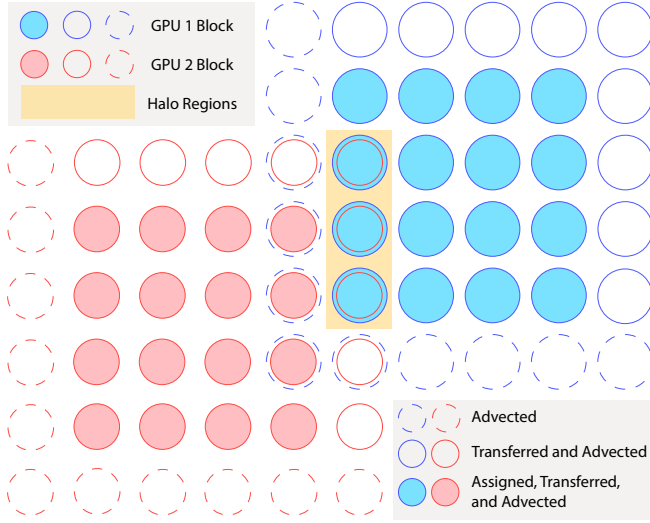
Fig. 10. Halo block tagging. We tag grid blocks with three labels: assigned, transferred, and advected. Assigned grid blocks are the blocks where particles are residing in. Transferred grid blocks contain the grid-nodes that particles may write to; e.g., with quadratic B-spline kernel, each particle may write to neighbor nodes within a three-cell distance. Advected grid blocks represent the blocks where particles may advect to after the G2P and the particle advection . The transferred and the advected grid blocks may contain no particles in the current time step. In the context of multi-GPU MPM, the partition from one device can overlap partitions from other devices. These overlapping regions ( i.e. , halo regions) may include all three types of grid blocks. The grid data in the halo regions should be shared and synchronized by the corresponding GPUs to ensure the execution correctness.
