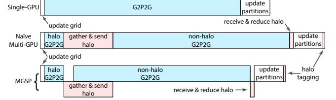
Fig. 9. Instruction pipelines. The additional operations in the multi-GPU MPM compared to the single-GPU MPM are displayed in red. By masking these halo-region-related data transfers with the execution of the G2P2G kernel, one can achieve more optimized scaling results with multi-GPUs.
