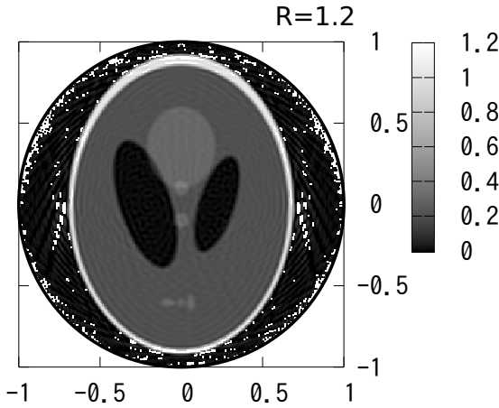
Fig. 8: Reconstruction Result by Proposed Method by Integral Path with K = 360 , N = 360 , M = 180 and Radius 1.2
