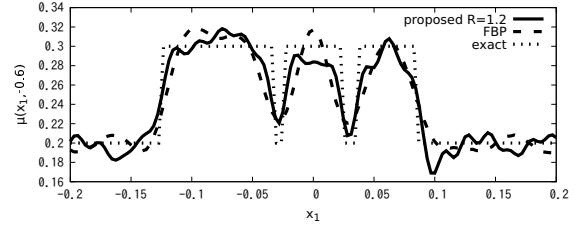
Fig. 15: Section of Locally Reconstructed \mu(x) (Fig. 13 and Fig. 14) on x_2 = -0.6
