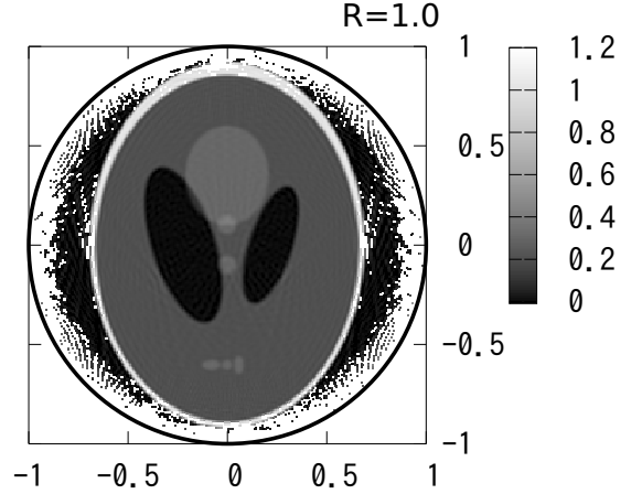
Fig. 6: Reconstruction Result by the Proposed Method by Integral Path with K = 360 , N = 360 , M = 180 and Radius 1.0
