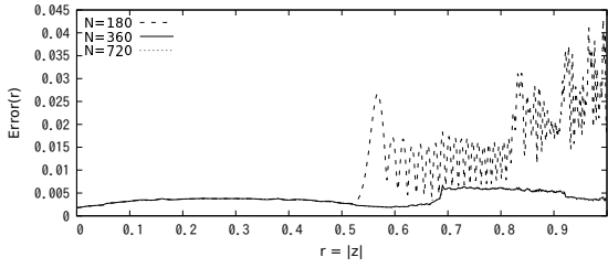
Fig. 11: Error Dependency on N (Number of Measurement Angles), with R = 1.1 , K = 360 , and M = 180
