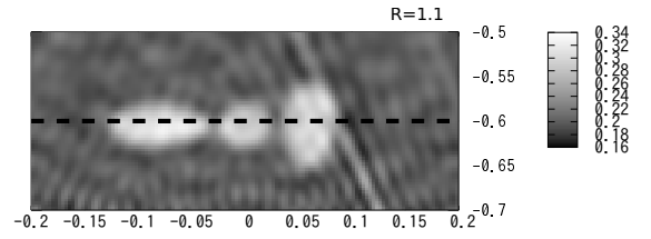
Fig. 14: Locally Reconstructed \mu(x) by Proposed Method in Rectangle [-0.2, 0.2] \times [-0.7, -0.5] . Section Along Dotted Line is Shown in Fig. 15
