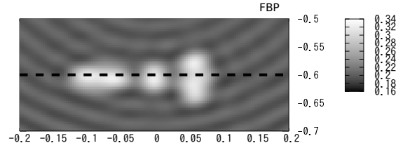
Fig. 13: Locally Reconstructed \mu(x) by Filtered Back-projection in Rectangle [-0.2, 0.2] \times [-0.7, -0.5] . Section Along Dotted Line is Shown in Fig. 15
