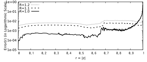
Fig. 9: Errors in U_1(z) Measured by (10)
