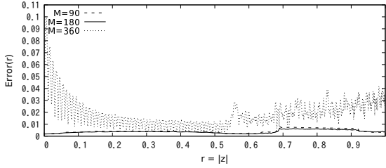
Fig. 12: Error Dependency on M (Truncation of Series), with R = 1.1 , K = 360 , and N = 360
