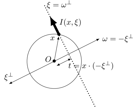
Fig. 4: Setting of Transport Equation (3) and Radon Transform
