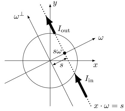
Fig. 3: Measurement of X-ray Intensity Transmitting D
