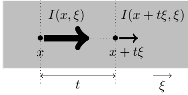
Fig. 1: Attenuation of Straight Forwarding X-ray
