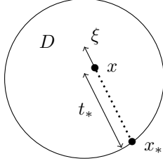
Fig. 2: Characteristic Line Passing x with \xi -direction and Its Initial Point x_* on the Boundary and Distance t_* = |x - x_*| .
