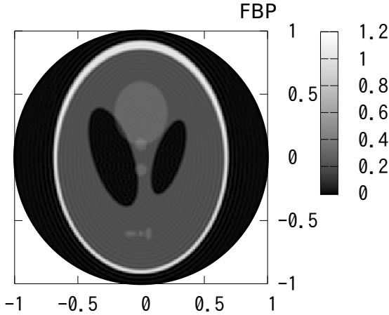
Fig. 5: Reconstruction Result by Filtered Back-projection with Linear Interpolation in P_w * h(s) at s = x \cdot \omega
