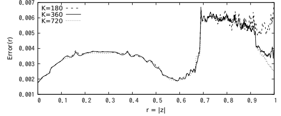
Fig. 10: Error Dependency on K (Number of Spatial Measurement Nodes), with R = 1.1 , N = 360 , and M = 180
