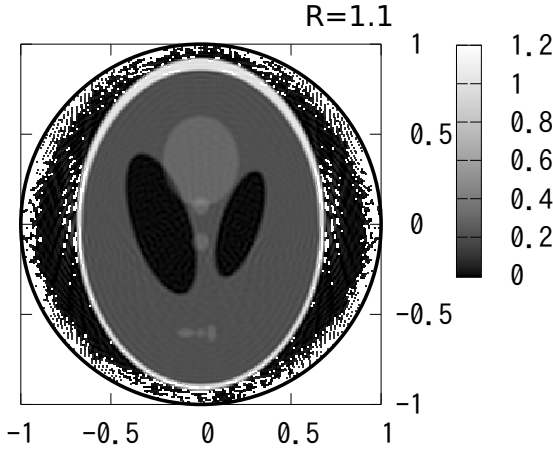
Fig. 7: Reconstruction Result by Proposed Method by Integral Path with K = 360 , N = 360 , M = 180 and Radius 1.1
