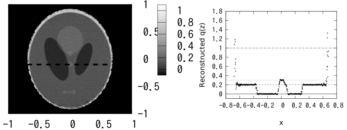
Figure 5: Reconstructed q_\ell by Algorithm FD [6] on \Omega (left) and its section on the dotted line (right)
