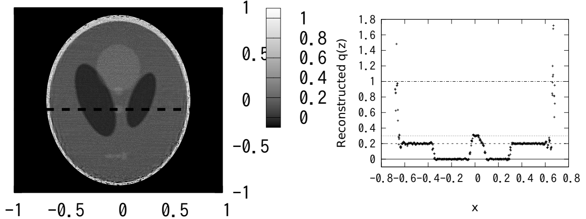
Figure 4: Reconstructed q_\ell by Algorithm P1 on \Omega (left) and its section on the dotted line (right)
