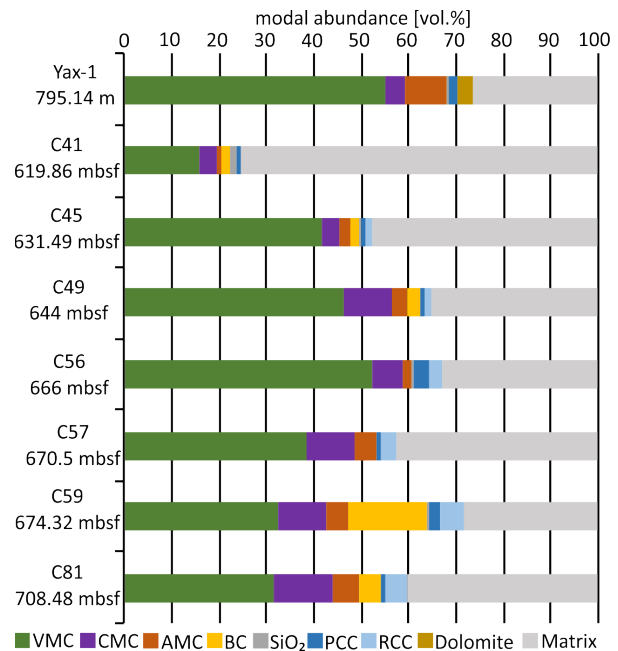
Fig. 1. Chicxulub sorted suevite modal composition.
