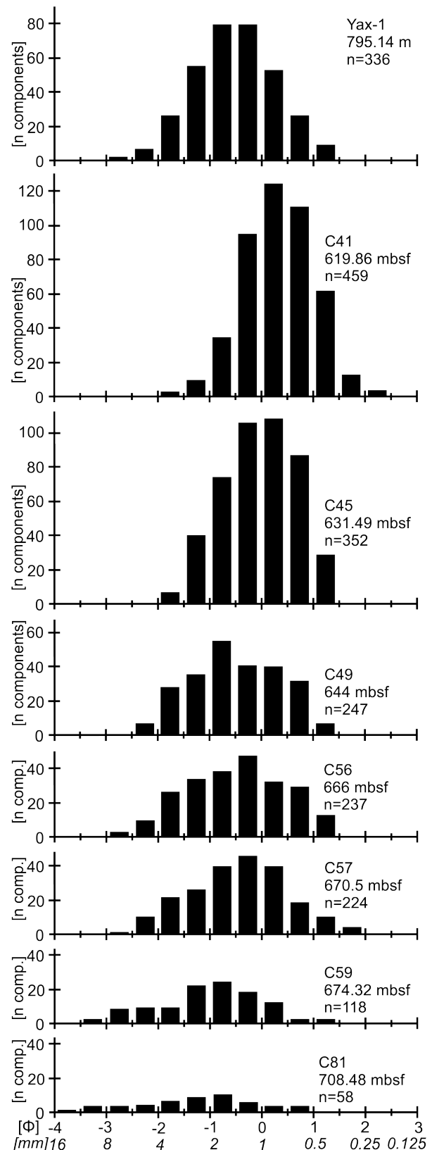
Fig. 2. Component size distributions of Chicxulub sorted suevite; \Phi is -\log_2 of component size.
