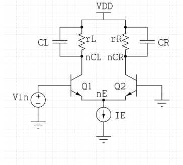
(a) Schematic.
