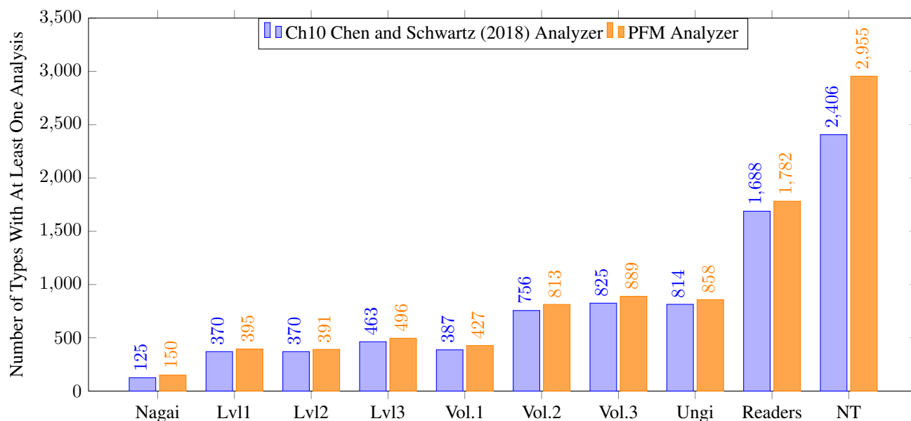
Figure 8: For each collection of texts in the Stories Test Set , depicts the number of types for which each analyzer returned at least one analysis.
