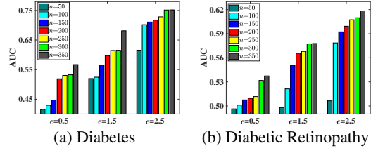
Figure 4: The AUC measurement of OffPairC.
