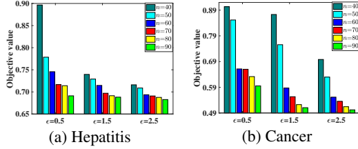
Figure 3: The objective value of OffPairStrC for AUC maximization.
