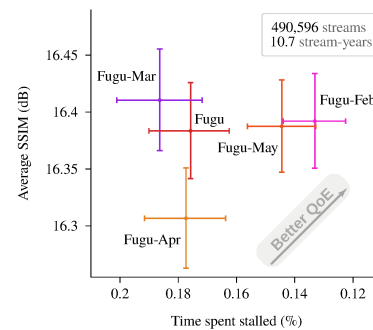
Figure 8: Fugu, which is retrained every day, did not outperform older versions of itself that were trained up to 11 months earlier. Our practice of daily retraining appears to be overkill.
