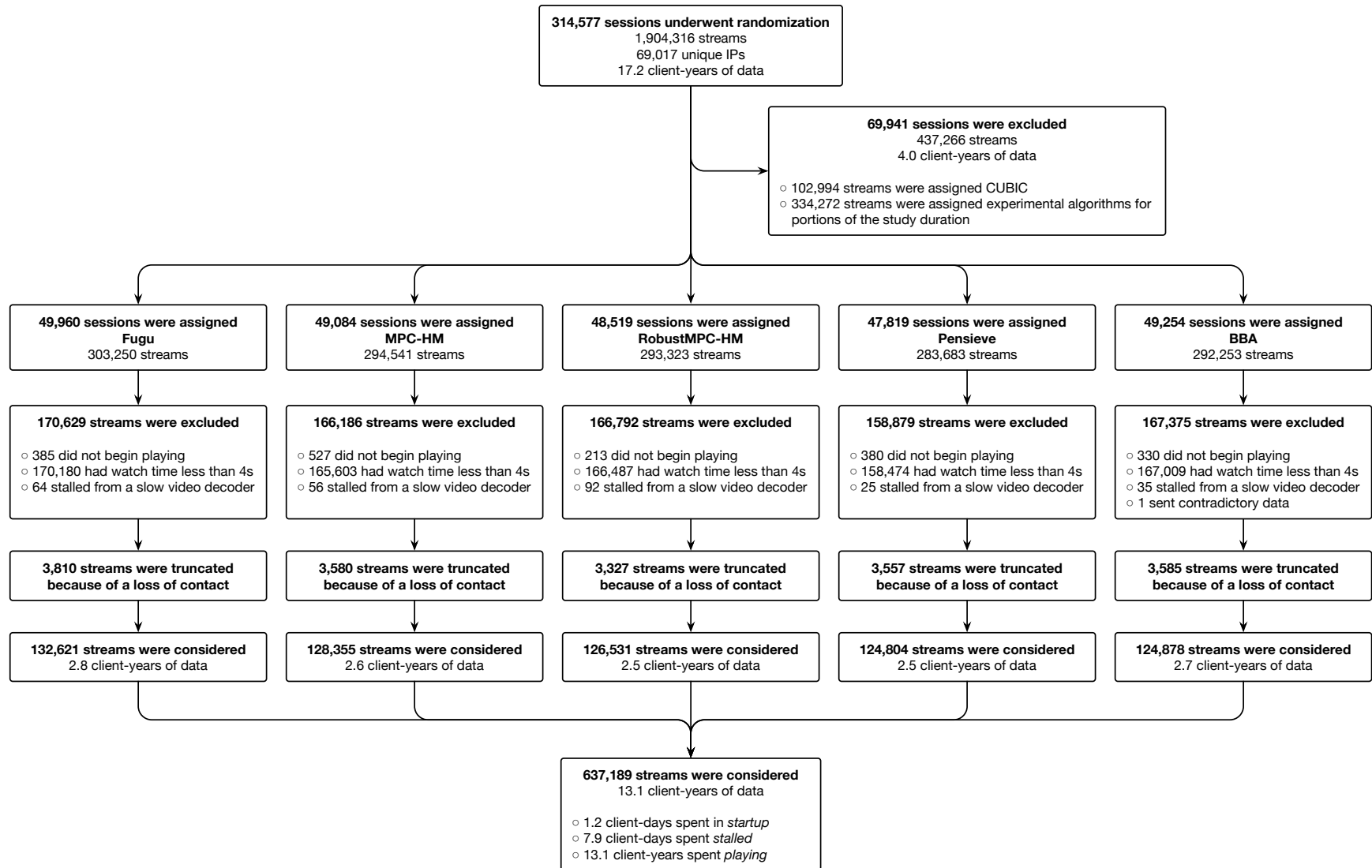
Figure A1: CONSORT-style diagram [35] of experimental flow for the primary results (Figures 1 and 9), obtained during the period Jan. 26–Aug. 7, 2019, and Aug. 30–Oct. 16, 2019. A “session” represents one visit to the Puffer video player and may contain many “streams.” Reloading starts a new session, but changing channels only starts a new stream and does not change TCP connections or ABR algorithms.
