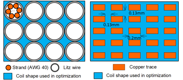
Fig. 2. Cross sections of equivalent macro coils of Litz wire and PCB stator windings used in 3D parametric models for optimization. Dimensions of PCB traces and the gap between them depend on the number of layers, overall thickness, finished copper, etc., and are closely related to PCB manufacturers.
