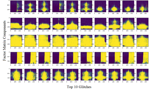
Figure 3: Each row in the figure represents the top-10 glitch instances from each component of the factor matrix obtained from CP/PARAFAC decomposition with rank 5. Observe that row 5 shows the cluster of loud Koi Fish type glitches isolated within the Extremely Loud class.
