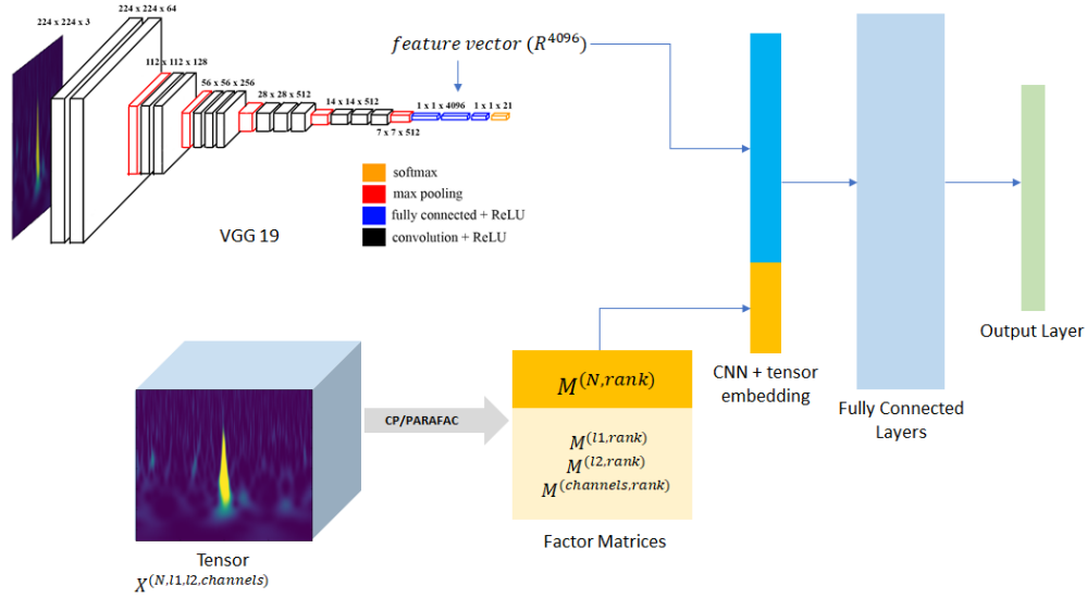
Figure 4: Block Diagram of Ensemble method which combines feature vectors from VGG19 fine-tuned on 10% of the labeled glitches and CP/PARAFAC decomposition of tensor representing all the glitches.
