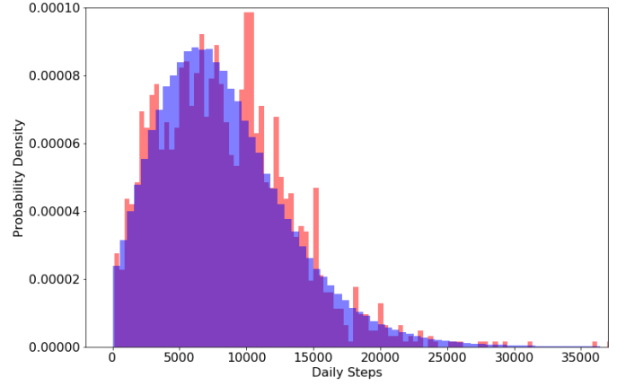
Fig. 2. Histogram (red) of daily step recordings collected from participants in a Mechanical Turk experiment [18] ( n = 1665 ) overlaid with a histogram (blue) of the steps generated by the pattern step simulator ( n = 500k ).
