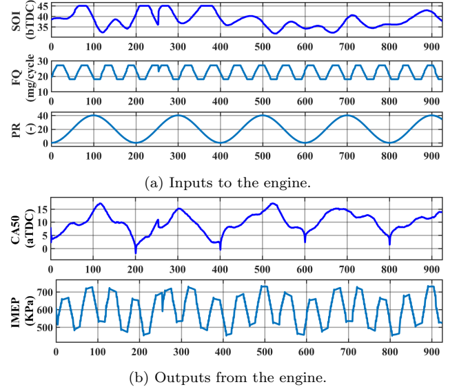
Fig. 2. Input/output data set used for LPV-SS model learning of RCCI engine.
