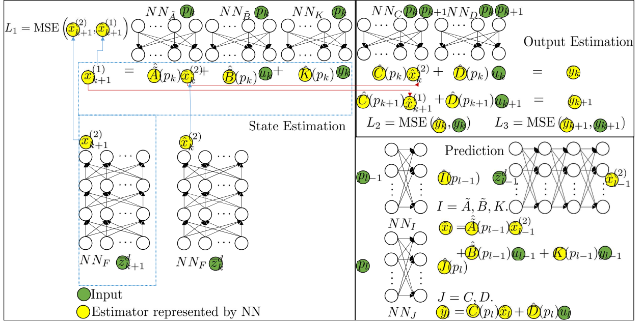
Fig. 1. The complete computing graph of SIME. NN_I ( I = \tilde{A}, \tilde{B}, K, C, D, F ) are used to distinguish neural networks. The green and yellow circles represent the inputs and outputs of their adjacent neural networks respectively (except for x_k^{(2)} and x_{k+1}^{(2)} which are computed by NN_F ). The red lines show the connections between computing graphs of state and output estimation modules.
