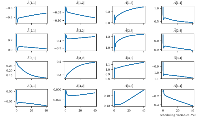
Fig. 4. The estimation of matrix functions as a function of p in the learned LPV-SS model (Take \hat{A} as an example). All the horizontal axes represent the scheduling variable PR . By approximating a smooth function for each matrix entry, the trained SIME model can predict the states and outputs of a system with high accuracy.
