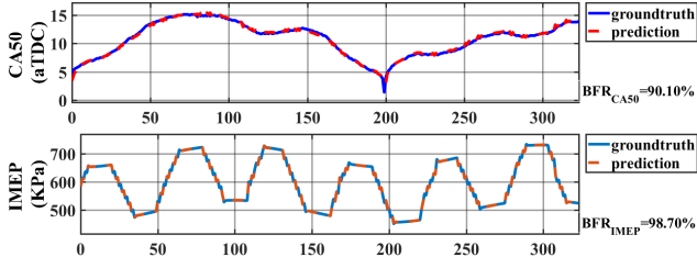
Fig. 3. The output response of the estimated LPV-SS model and the response of the original system on the validation data set.
