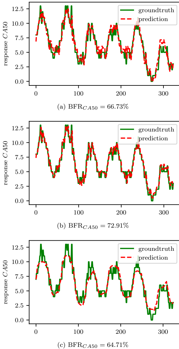
Fig. 5. Output estimation using identified LPV-SS model on real RCCI engine data with full state measurements. Solid and dashed lines show respectively the measurement and model prediction. Subplot (a) shows the results of regression using ANN without regularization; subplot (b) shows the results of LPV-SS regression using ANN with regularization; subplot (c) shows the result of our previous work (Irdmoussa et al., 2019).
