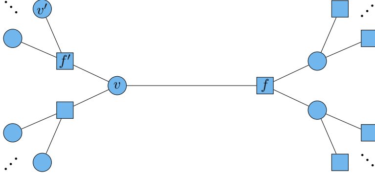
Figure 2: The sub-tree \mathcal{T}_{v \rightarrow f} .
