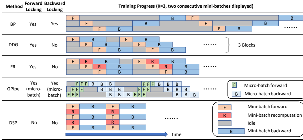
Figure 1. Sketches of different methods with three blocks. The forward and recombination are overlapped in DSP.
