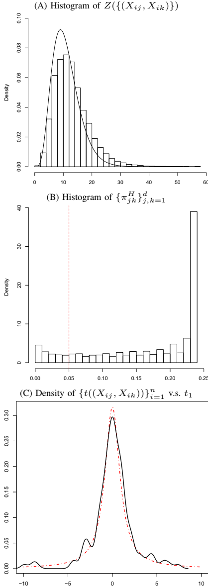
Fig. 5. (A) The histogram of Z(\{(X_{ij}, X_{ik})\}) for the pairs of genes for the prostate tumor and the curve is the density function of \chi^2_{11} ; (B) The histogram of the Holm's adjusted p-values for the prostate tumor and the red dashed line is the significance level \alpha = 5\% ; (C) The estimated density of \{t((X_{ij}^*, X_{ik}^*))\}_{i=1}^n (black solid line) versus the density of t_1 (red dashed line) for the pair of genes with largest p-value of the statistic Z(\{(X_{ij}, X_{ik})\}) .
