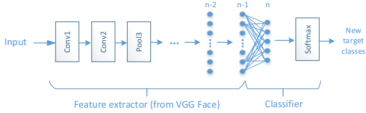
Figure 2: Transfer learning on VGG Face
