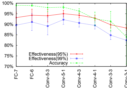
(a) Effect of re-training more layers
