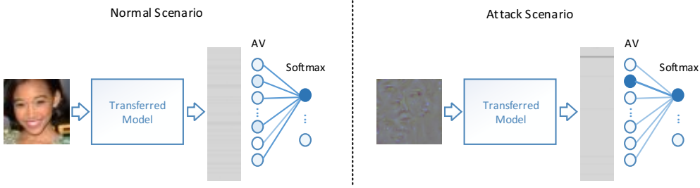
Figure 1: Example of activation vector and how the Softmax layer responds. The image on the left shows the activation vector of a natural face in the training set. The Softmax layer performs Softmax operation over the linear combination of such activation vectors and assigns high confidence to the corresponding class. The target-agnostic image (the image on the right) is crafted such that it activates one neuron in activation vector with extremely large value and all others are almost zero. Such activation vector also fools the softmax layer to produce output with high confidence. Due to the lack of space, we only show the first 400 neurons of the activation vector.
