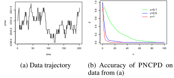
Figure 1. Real data and accuracy results.
