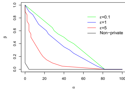
Figure 3. Empirical accuracy \beta = \Pr[|\tilde{t} - t^*| > \alpha] of PNCPD for drift change detection.
